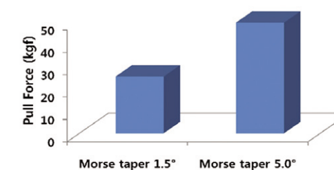
• Fig. 3. The result of pull-out test of fixtures with Morse taper 1,5° (B-company fixture) and Morse taper 5° (AnyRidge fixture).
